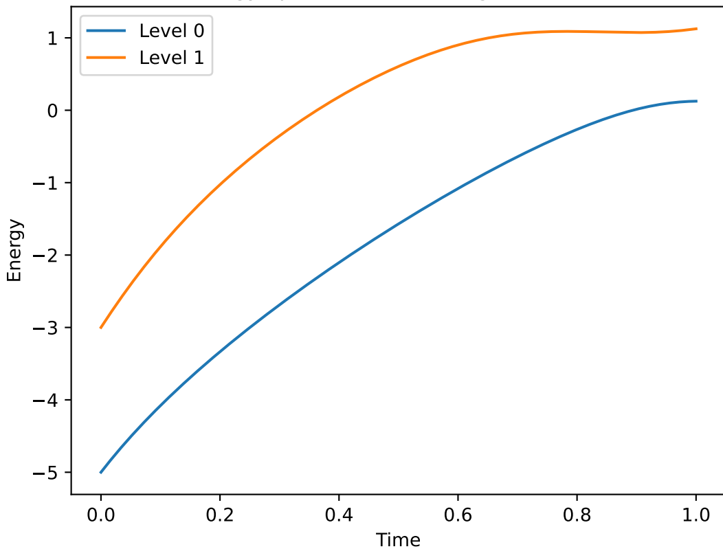
Energy spectrum for n=5 , \gamma=1.0
