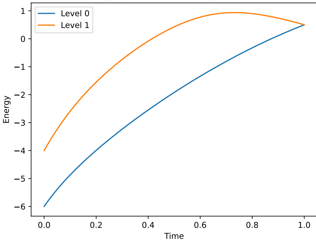
Energy spectrum for n=6 , \gamma=1.0
