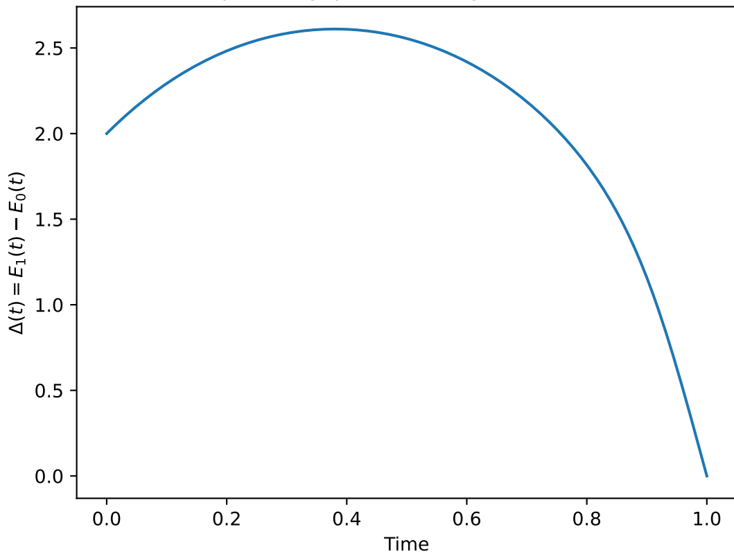
Spectral gap for n=12 , \gamma=1.0
