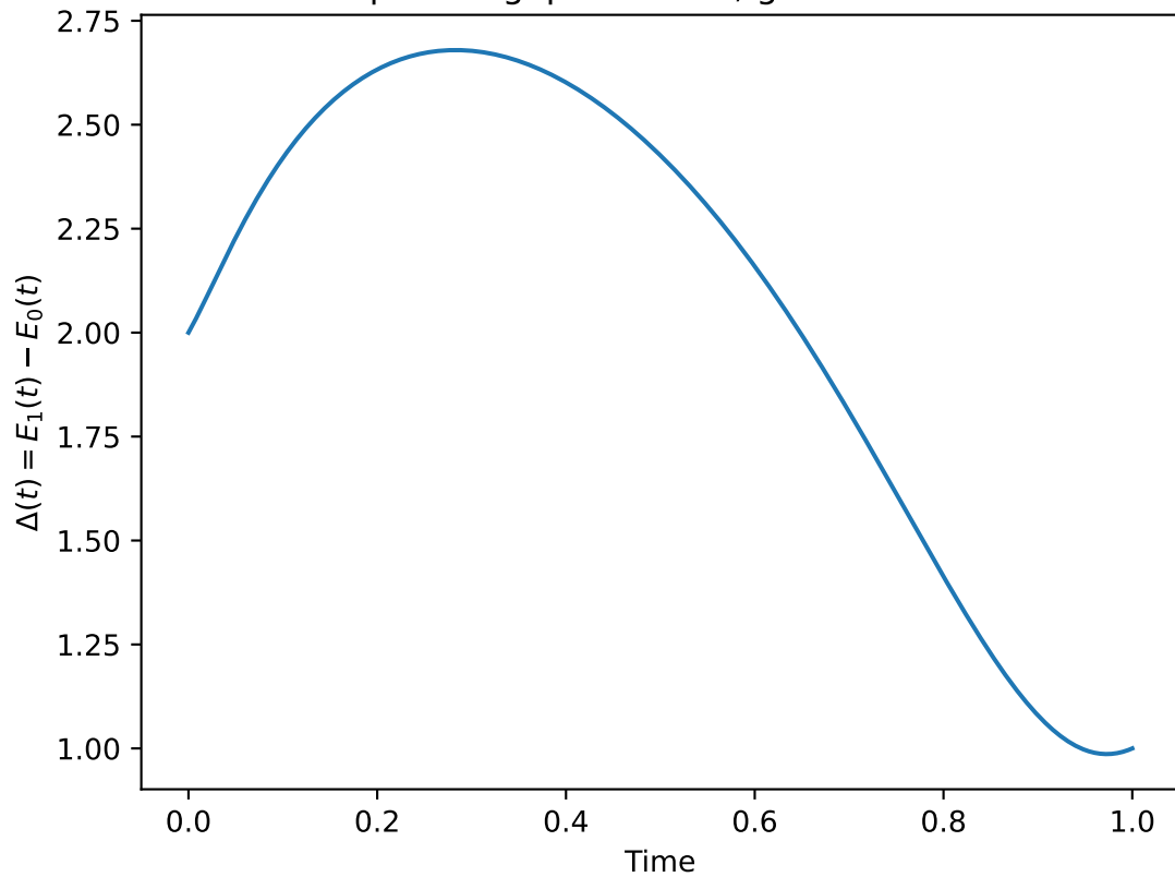
Spectral gap for n=13, gamma=1.0
