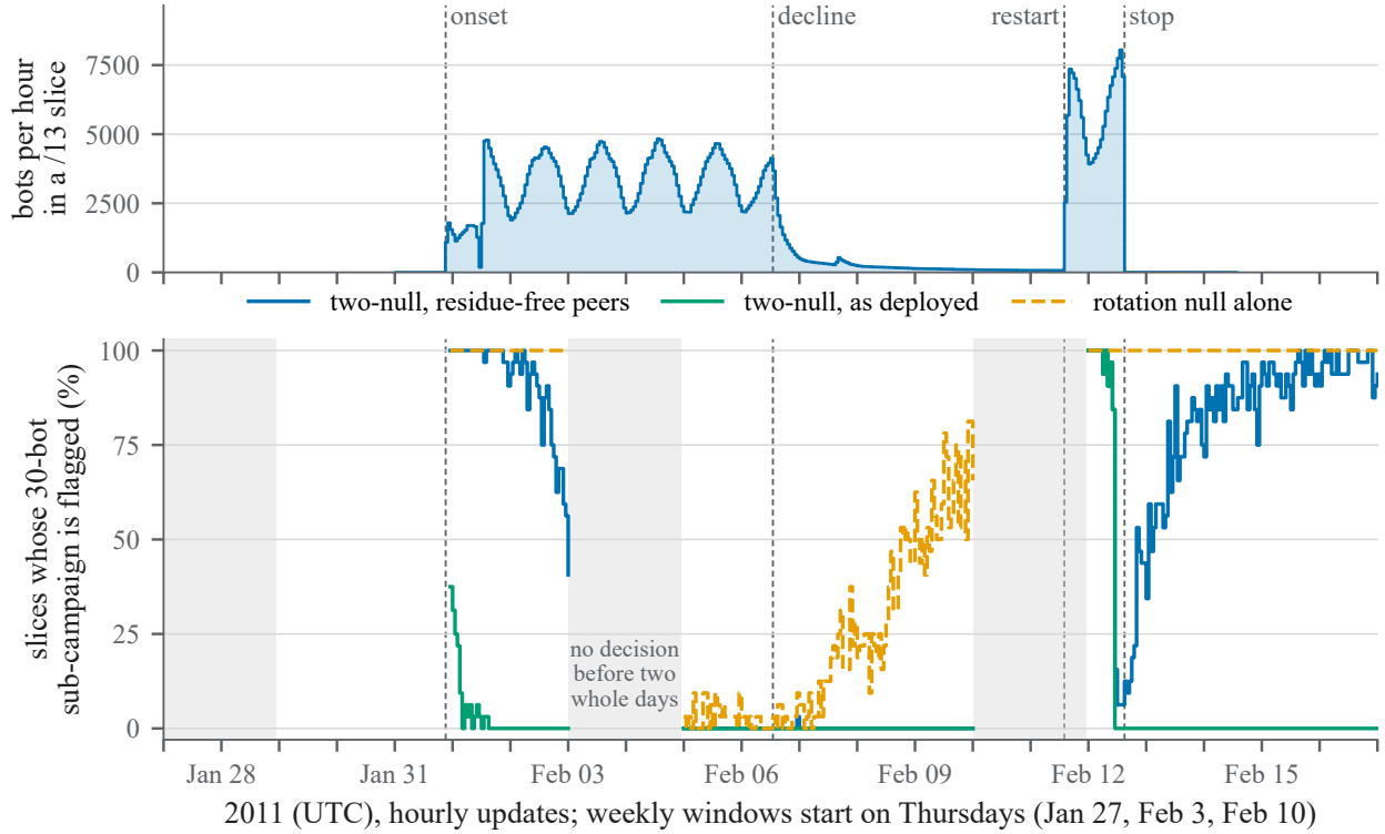
Figure 2: Hourly replay in the deployment mode. Top: as in Fig. 1. Bottom: share of the 32 slices whose 30-bot sub-campaign is flagged at each hourly update of the three Thursday windows; shaded: the first two days of each window, when no decision is made.
