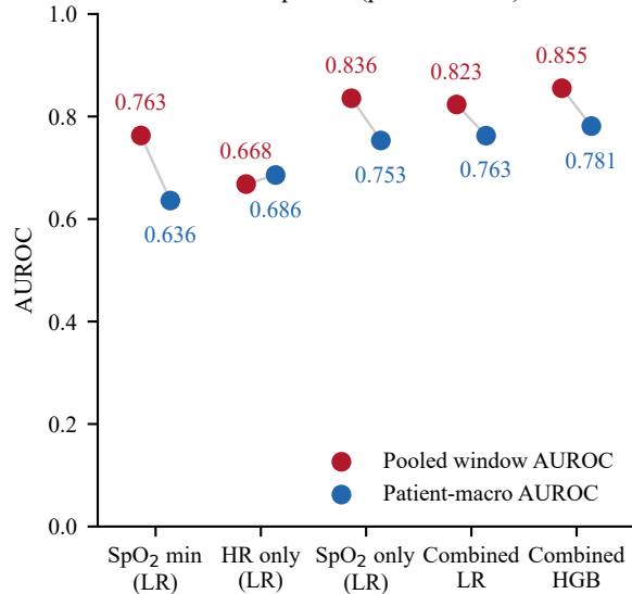
Pooled vs within-patient (patient-macro) AUROC
