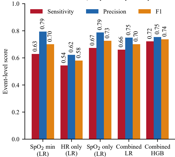
Event-level detection (many-to-many overlap matching)
