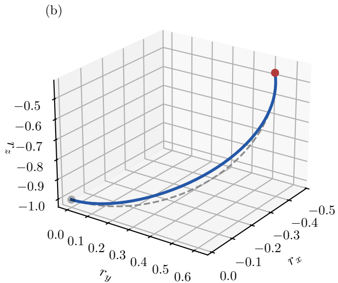
Induced stationary-state path
