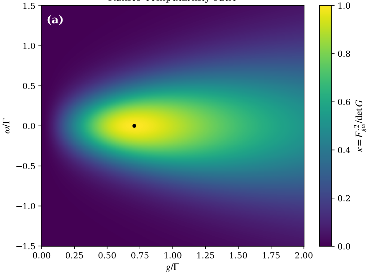
Kähler compatibility ratio
