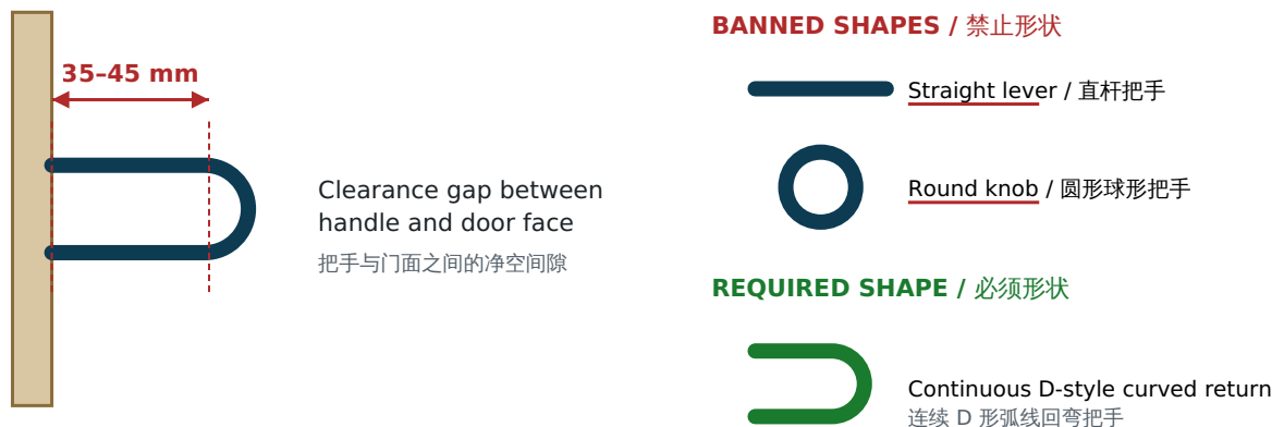
Figure 5 — Handle clearance dimension and required D-style shape / 图5：把手净空尺寸与必须的D形把手样式
