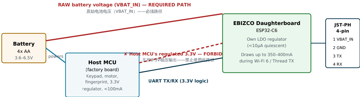
Figure 6 — Power & signal architecture: the daughterboard draws power directly from the raw battery, never from the host MCU's 3.3V rail / 图6：电源与信号架构——子板必须直接从电池取电，绝不可使用主控的3.3V输出
