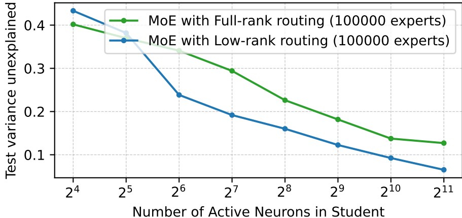
Unexplained fraction of variance when distilling middle MLP layer of Pythia-410M
