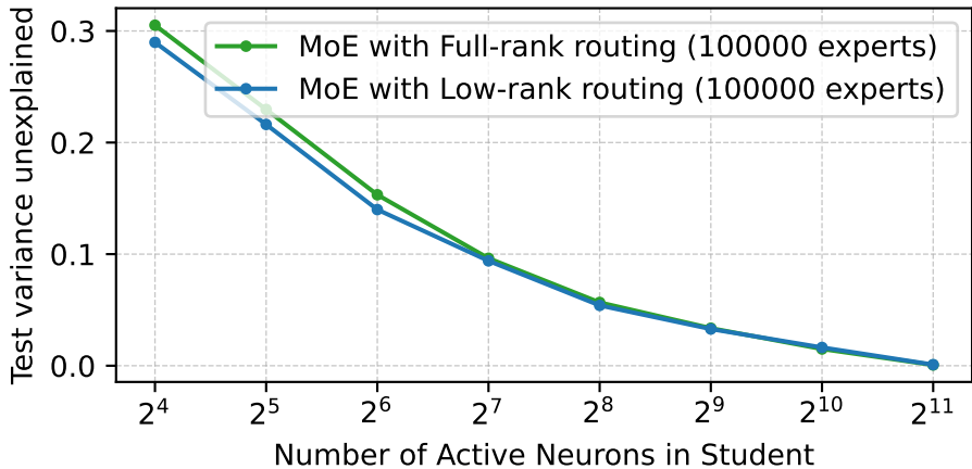
Unexplained fraction of variance when distilling middle MLP layer of Pythia-70M (Gaussian data)
