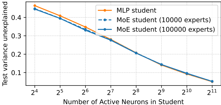
Unexplained fraction of variance when distilling middle MLP layer of Pythia-410M (Gaussian data)
