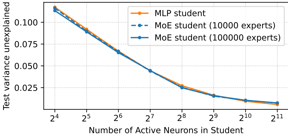
Unexplained fraction of variance when distilling middle MLP layer of Gemma-3-270M (Gaussian data)
