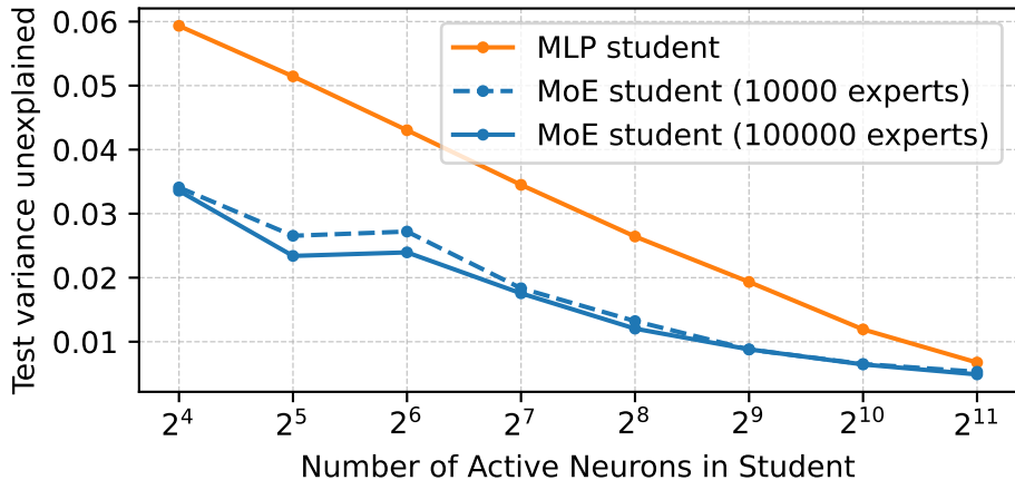
Unexplained fraction of variance when distilling middle MLP layer of Gemma-3-270M
