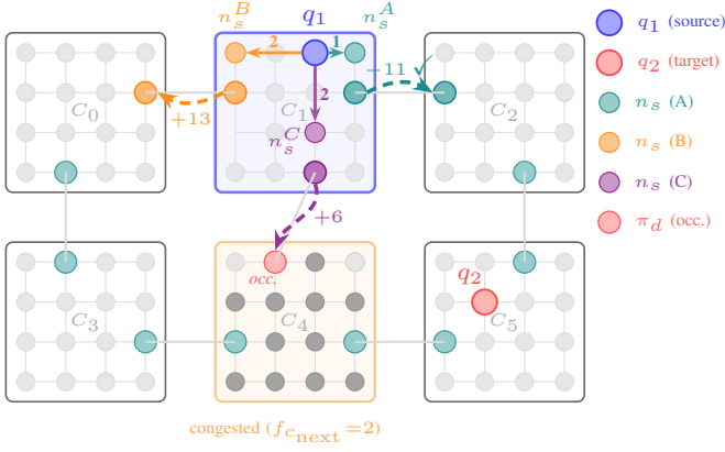
Fig. 4. How dSABRE chooses where to teleport a qubit. A cross-core gate g=(q_1, q_2) is pending, q_1 in C_1 (blue border) and q_2 in C_5 ; the router scores the three links leaving C_1 and takes the cheapest by Eq. (7). Executing one takes three steps: an occupied port is evacuated, intra-core SWAPs move q_1 to the staging slot n_s (count on the solid arrow), and a teleport along (\pi_s, \pi_d) carries it into the next core (dashed arc, annotated with the score s ). Candidates A, B, C match Table II row by row; C_4 's orange border marks only two free slots, and its red port occ must be evacuated—so C pays d_{\text{prep}}=3 against the two SWAPs on its arrow.
