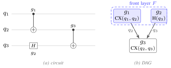
Fig. 1. DAG for a three-gate circuit on qubits q_1, q_2, q_3 . CX(q_1, q_2) and H(q_3) share no qubit and have no incoming edges, so both appear in the initial front layer F = \{g_1, g_2\} and may execute in parallel. CX(q_2, q_3) depends on both via qubits q_2 and q_3 ; it enters F only after g_1 and g_2 have been executed. Circuit depth is 2 (two sequential layers).
