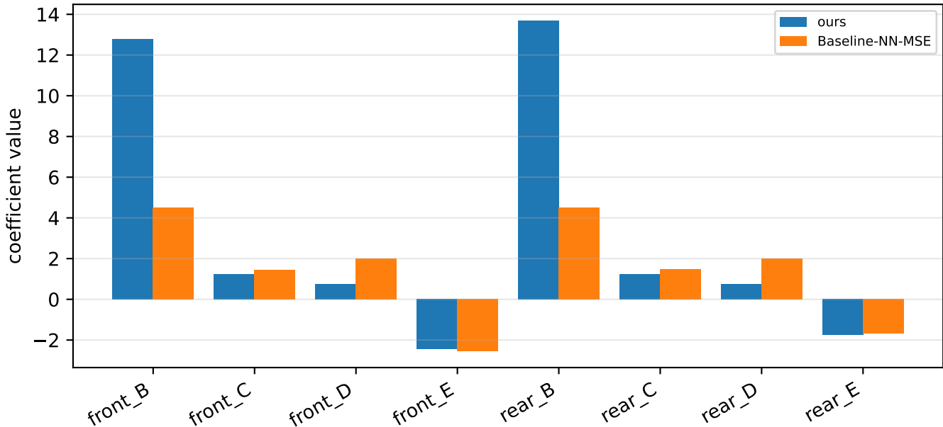
Identified Magic Formula coefficients
