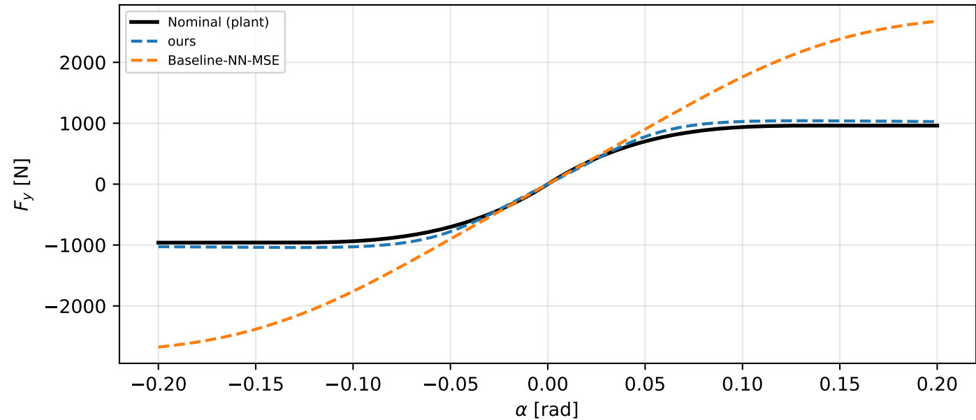
Rear axle
