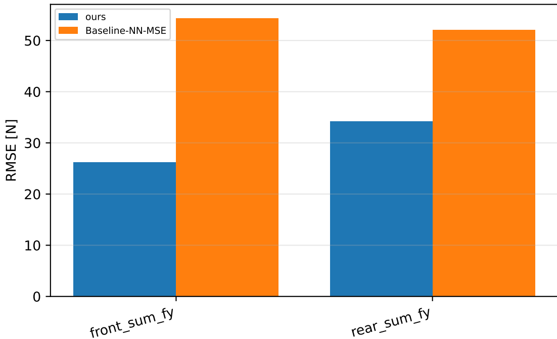
Tire lateral force: model accuracy per axle
