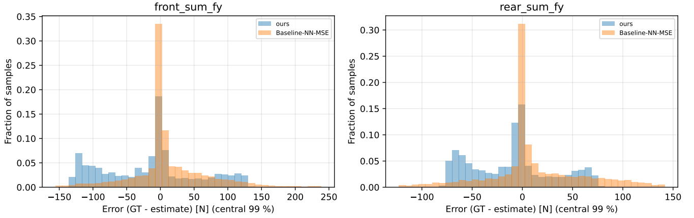
Fig. 4. Distribution of the axle lateral-force error (truth minus estimate), shared bin edges over the pooled central 99% and normalised to the sample count of each run. Both are centred; the inherited configuration buys its lower front RMSE with the heavier tail (maximum absolute error 215 N against 138 N front, 223 N against 85 N rear).
