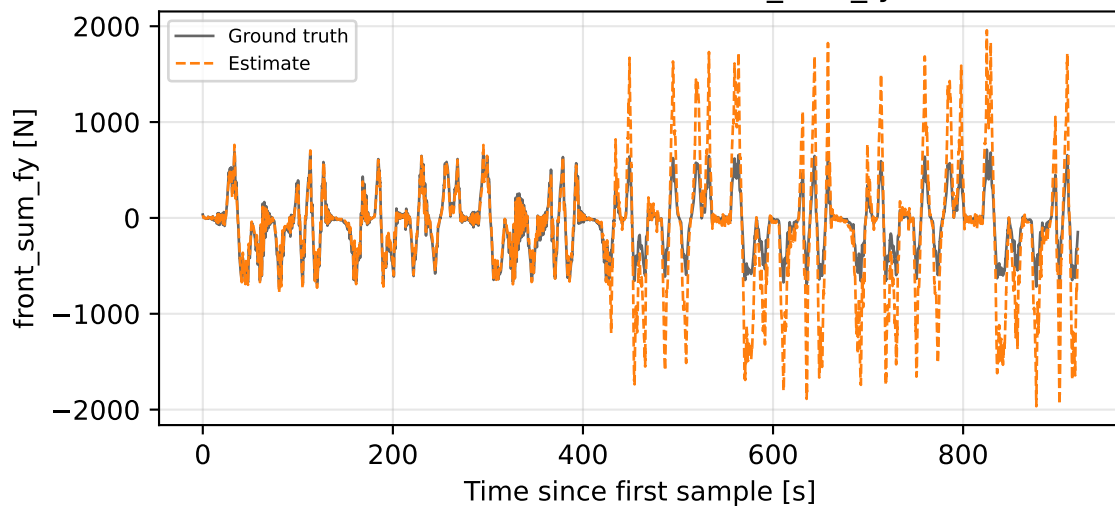
Baseline-NN-MSE - front_sum_fy
