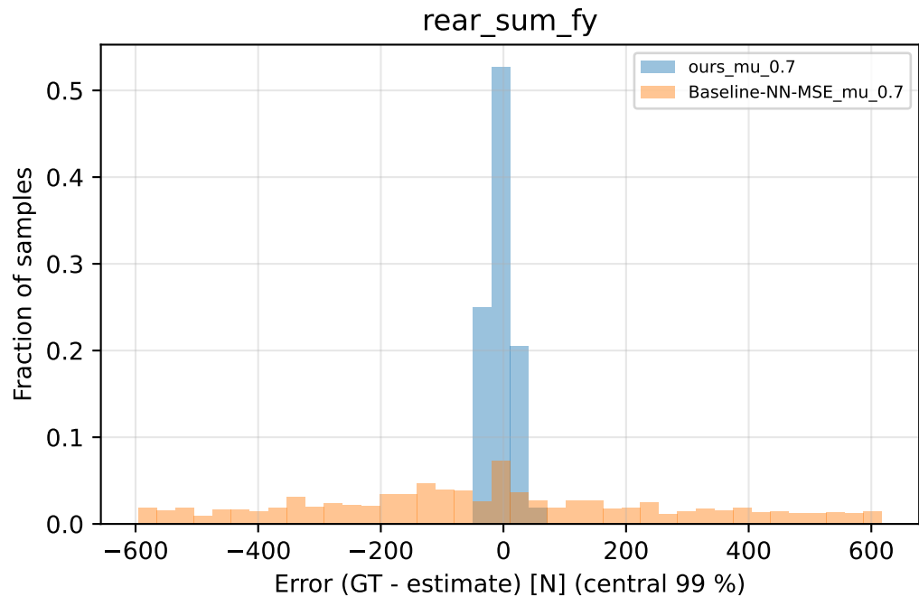
Tire lateral force error distribution by scenario
