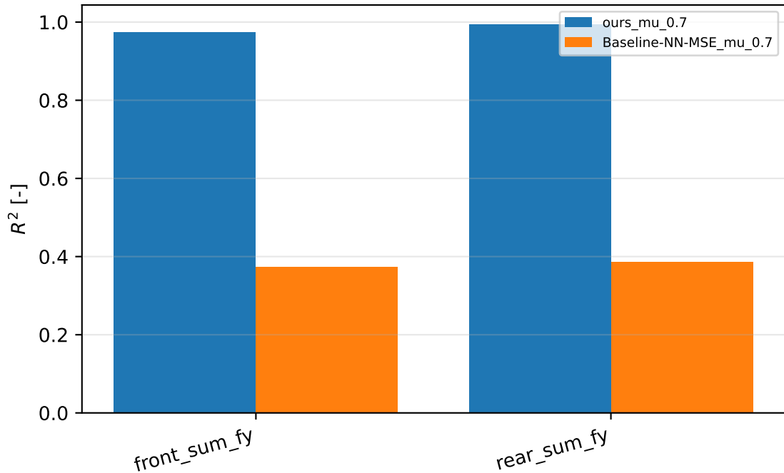
Tire lateral force: R^2 per axle
