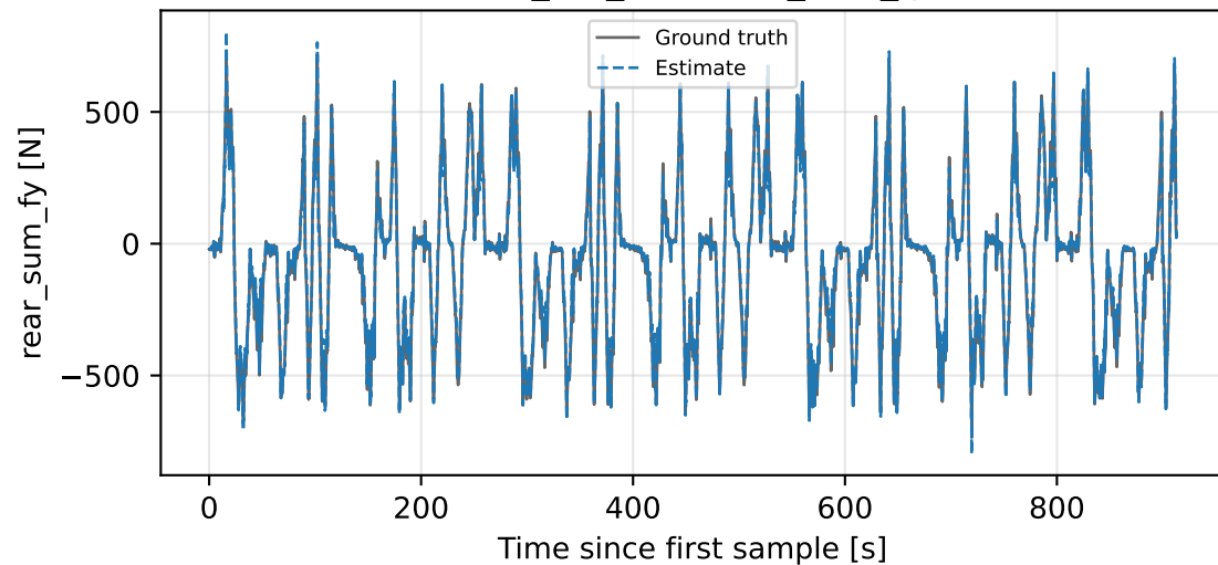
Baseline-NN-MSE_mu_0.7 - rear_sum_fy
