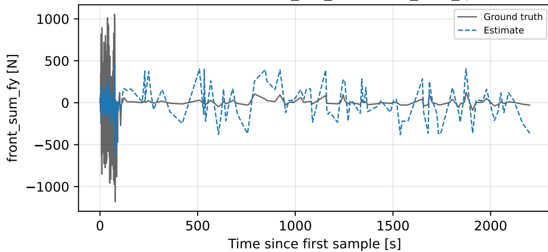
Baseline-NN-MSE_mu_0.7 - front_sum_fy
