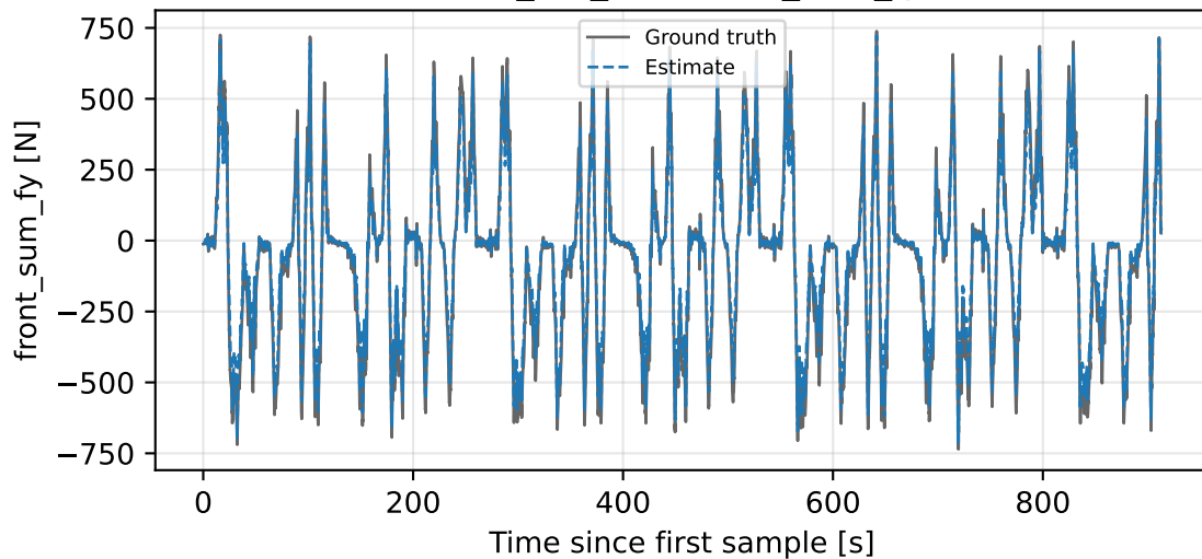
Baseline-NN-MSE_mu_0.7 - front_sum_fy
