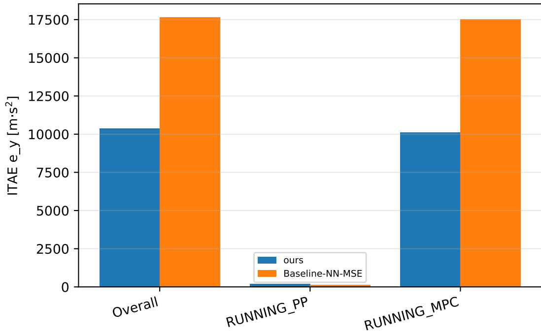
ITAE of lateral error by active controller
