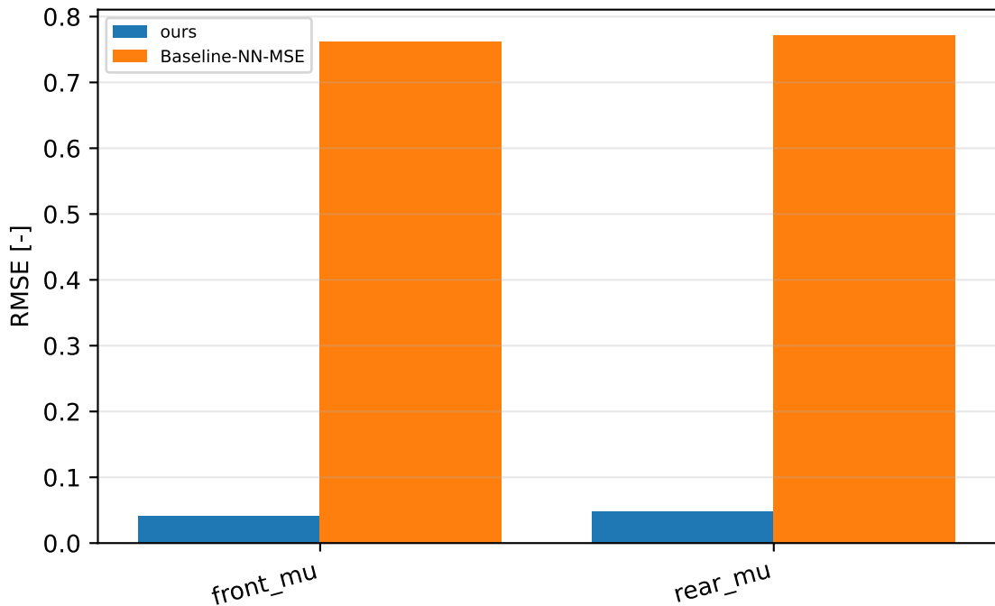
Peak friction: identified D against the simulator
