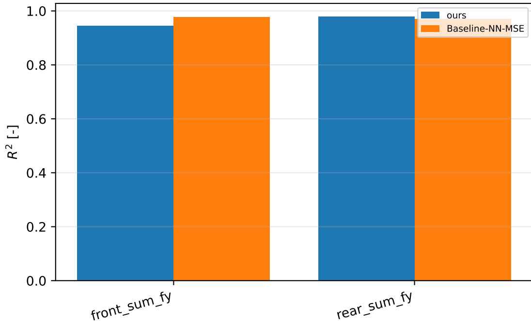
Tire lateral force: R^2 per axle
