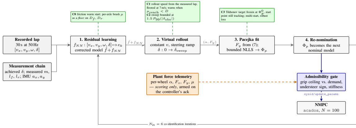
Fig. 2. The identification pipeline. Recorded lap data trains the residual network, the corrected model is rolled out through a synthetic steering sweep, Pacejka coefficients are fitted to that sweep, and the fit becomes the next nominal model under relaxation. Green marks this paper's changes: the friction warm start (Section V-E2), the excitation-aware rollout speed and extrapolation-bounded sweep (Sections V-B–V-C), the frozen regularisation target of (12) and the relaxed update of (14). Blue is the gated controller interface (Section VII); orange is the plant's per-wheel force telemetry, which scores the result and never enters the loop.
