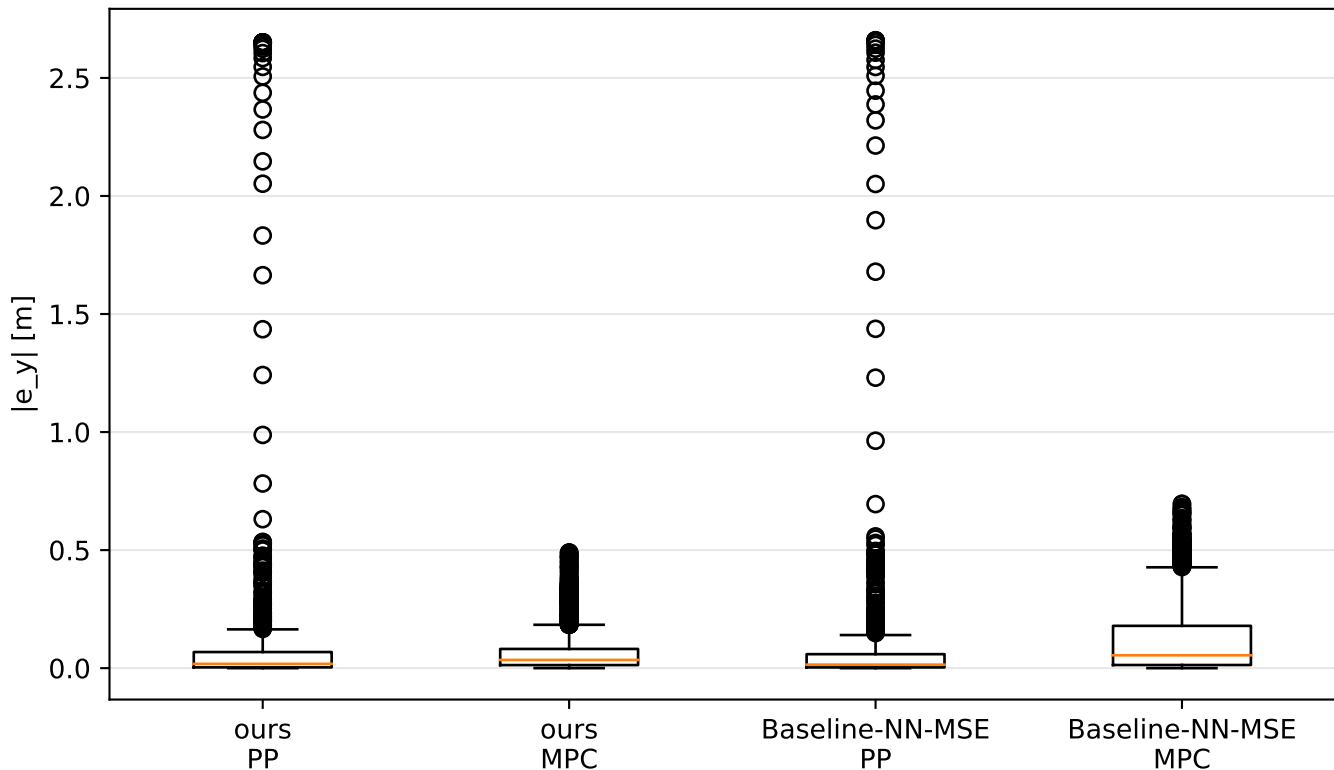
Lateral tracking error by scenario and active controller
