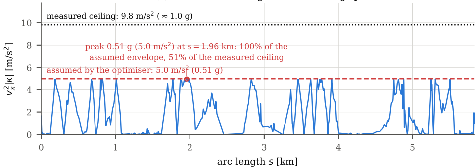
(c) lateral demand against available grip
