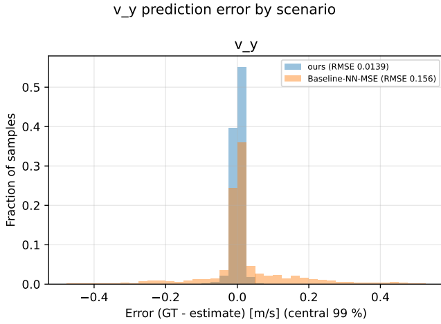
Fig. 7. Lateral-velocity prediction error (truth minus estimate). The two corrected configuration is an order of magnitude tighter on this channel (0.014 m/s against 0.156 m/s RMSE), and neither model beats its own persistence baseline.
