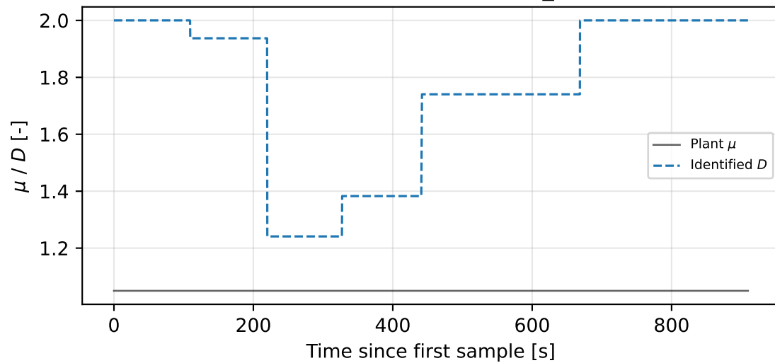
Baseline-NN-MSE - front_mu
