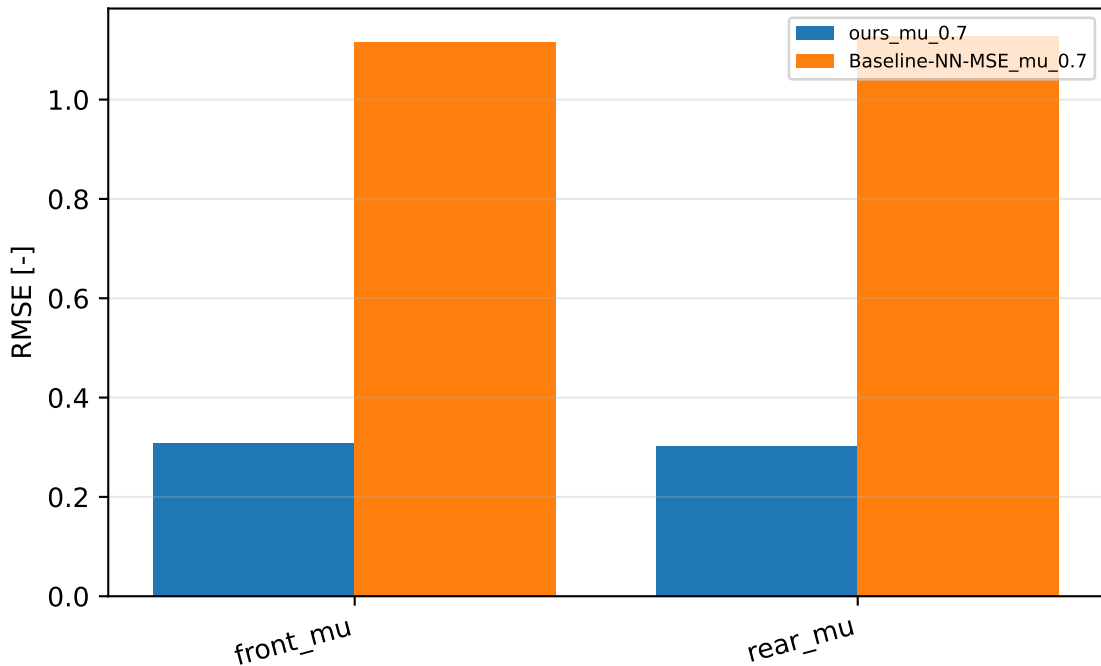
Peak friction: identified D against the simulator
