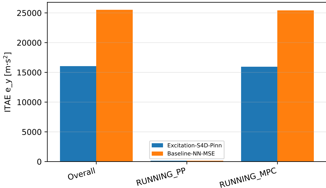
ITAE of lateral error by active controller
