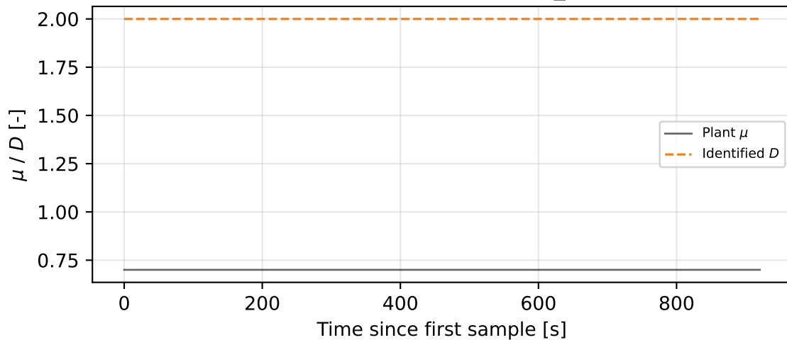
Baseline-NN-MSE - front_mu
