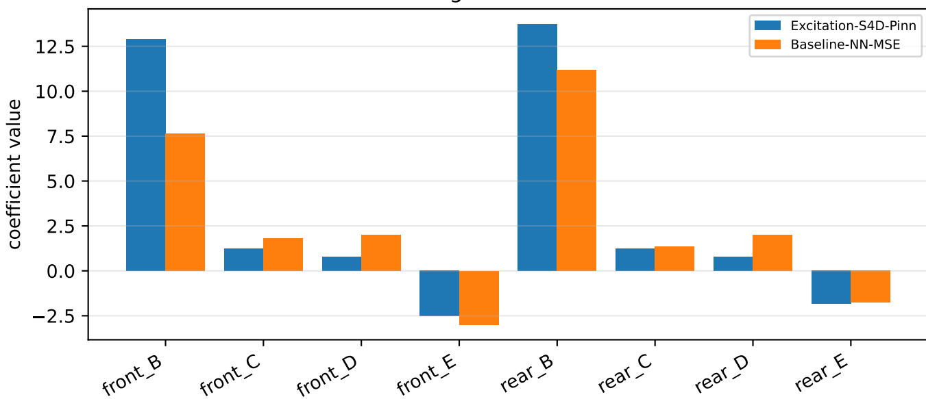
Identified Magic Formula coefficients
