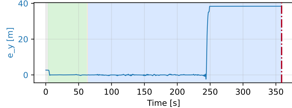
Baseline-NN-MSE-decay-mu
