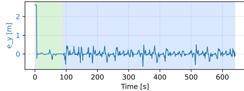
Baseline-NN-MSE-decay-mu
