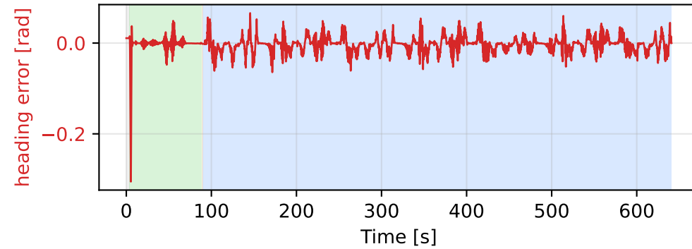
Heading tracking error
