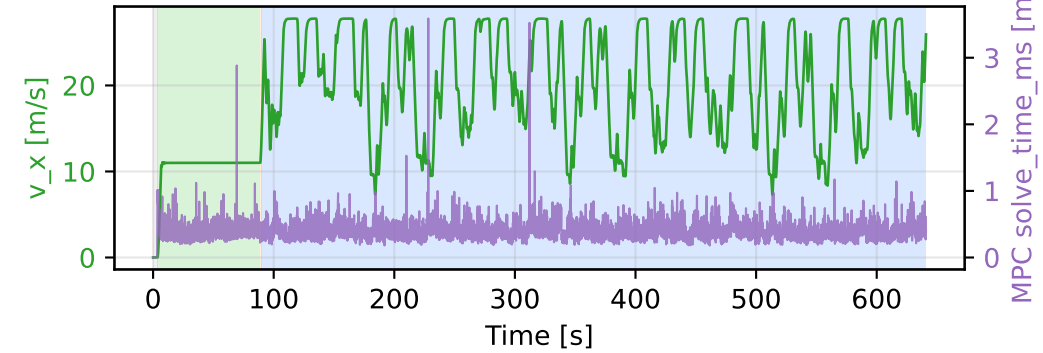
Speed profile vs. MPC compute cost
