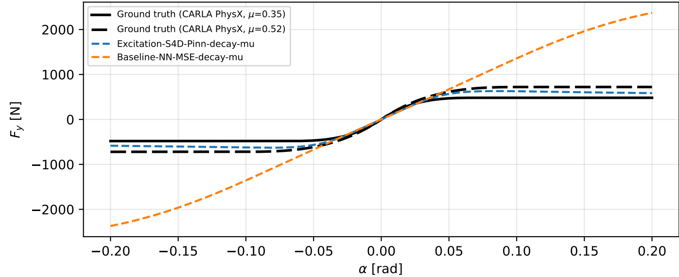
Rear axle
