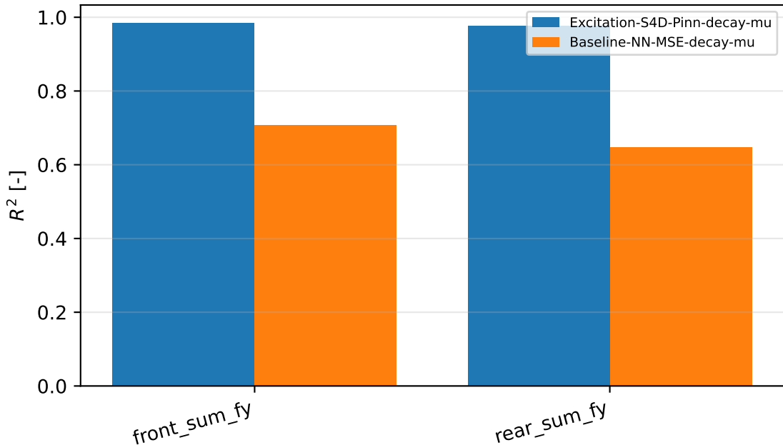
Tire lateral force: R^2 per axle
