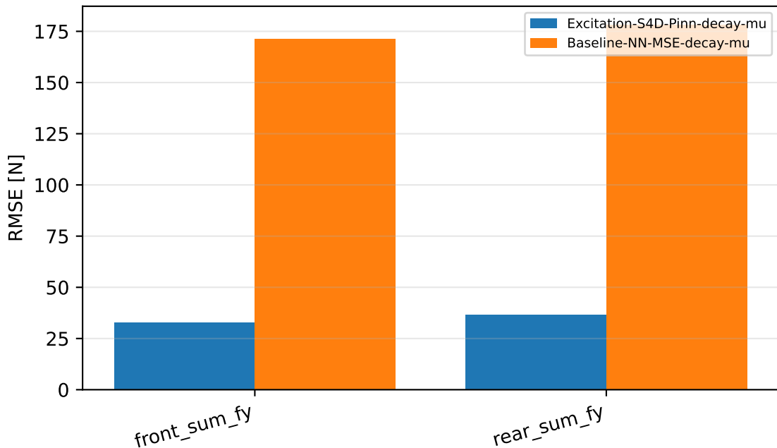
Tire lateral force: model accuracy per axle
