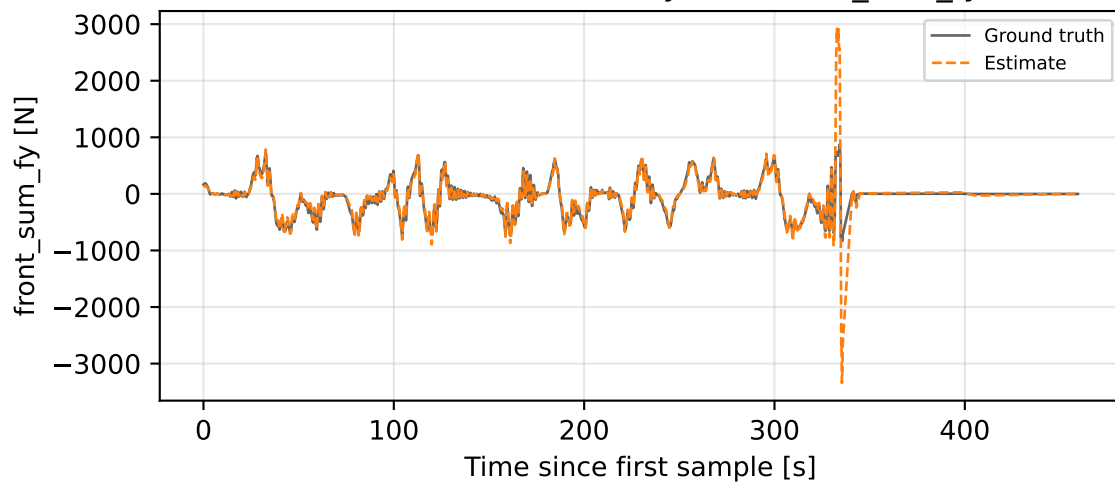
Baseline-NN-MSE-decay-mu - front_sum_fy
