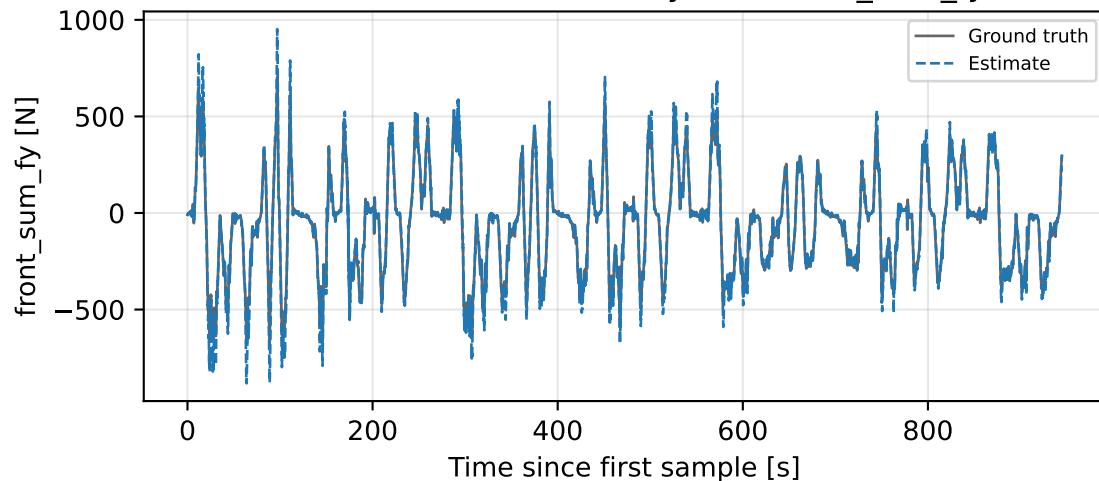
Baseline-NN-MSE-decay-mu - front_sum_fy
