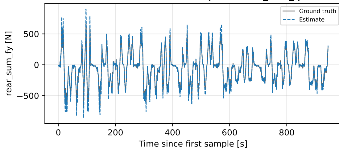
Baseline-NN-MSE-decay-mu - rear_sum_fy
