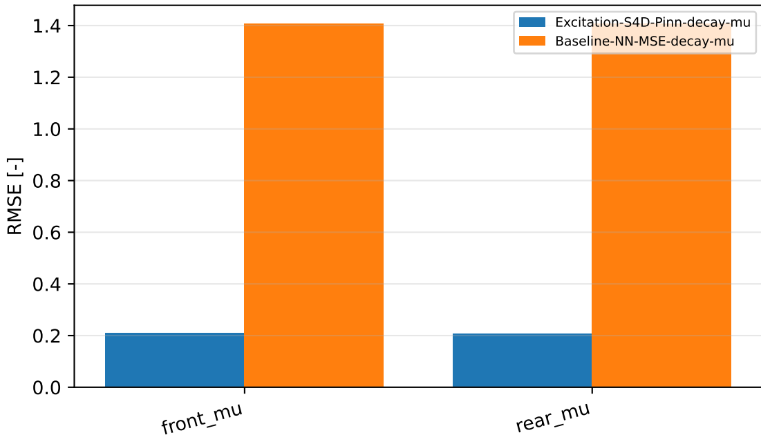
Peak friction: identified D against the simulator
