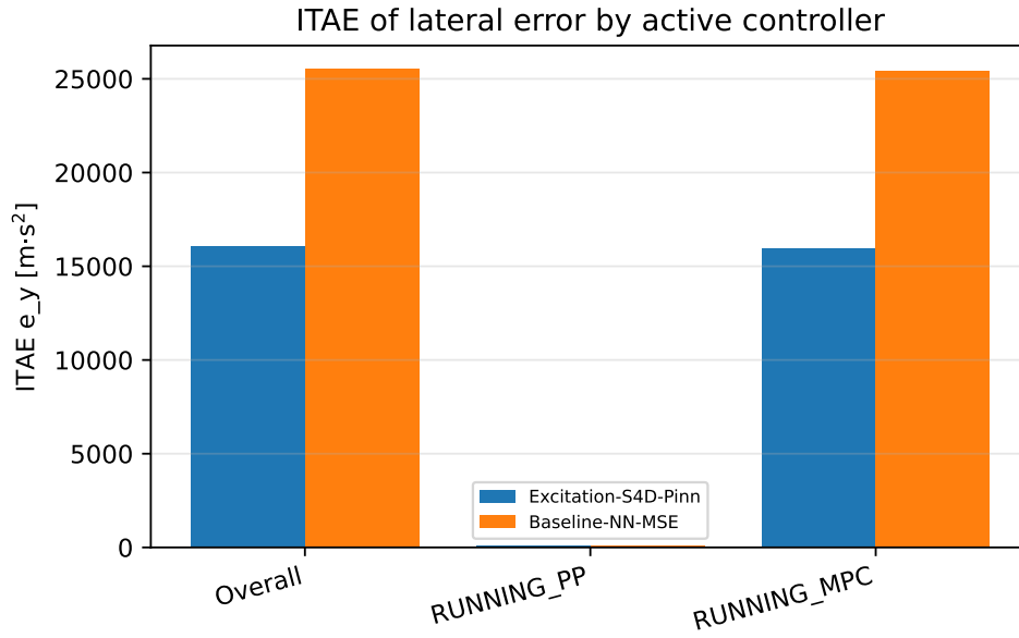
Fig. S11 ITAE of the lateral error, overall and split by the active controller. The pure-pursuit phases agree to 3% and are two orders of magnitude smaller, so the whole difference sits in the MPC phase, where the identified model is in the loop.
