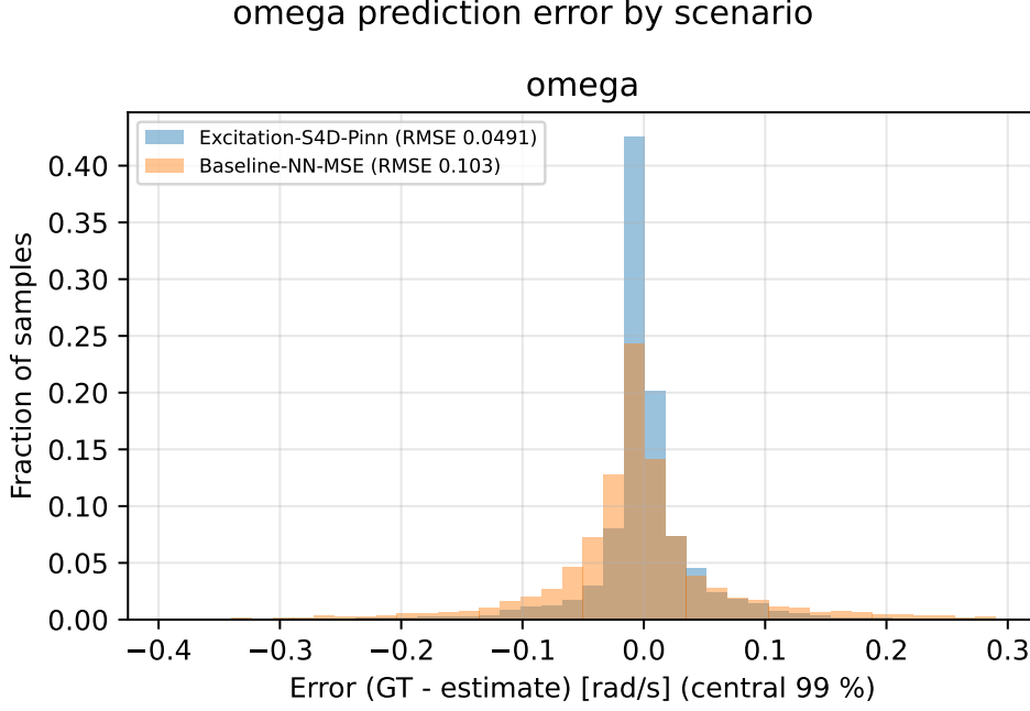
Fig. S8 Yaw-rate prediction error (truth minus estimate). The difference between the configurations is tail mass, not centre.
