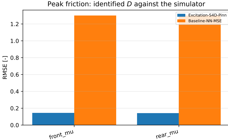
Fig. S2 Peak-friction error per axle against the effective coefficient the simulator reports per wheel, on the static \mu = 0.70 surface. The corrected configuration’s error is an order of magnitude smaller on both axes (0.145 and 0.142 against 1.300 on both, whole-run RMSE, and 0.078 once its friction gate has released); the inherited configuration’s error comes from a coefficient parked on its upper bound for the entire run rather than from a mis-estimate.
