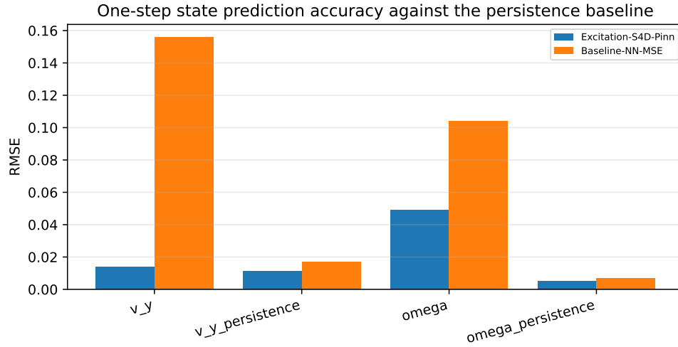
Fig. S6 One-step prediction RMSE for v_y and \omega against the persistence baseline of the same run. Neither identified model beats persistence at the 0.035 s model step.
