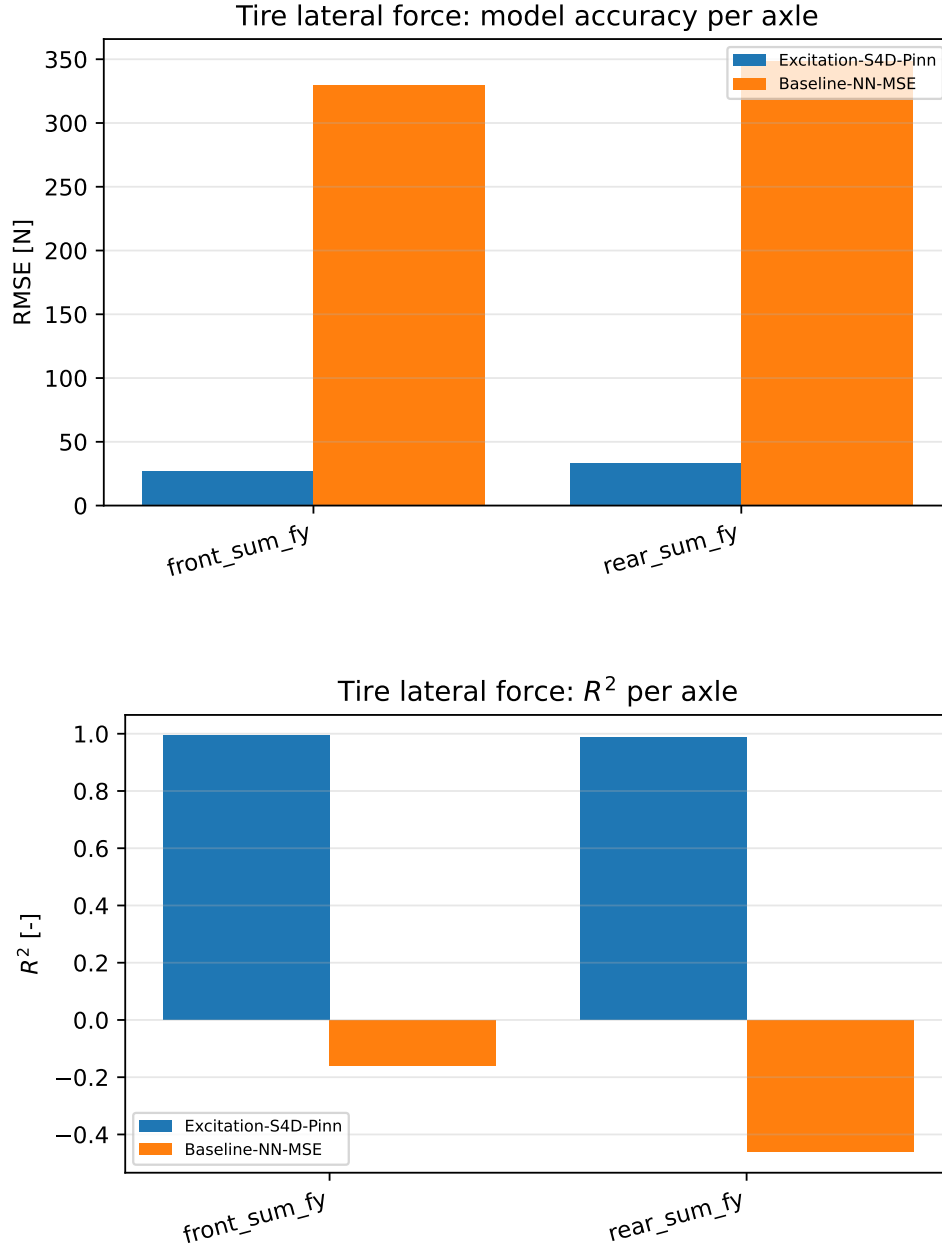
Fig. S3 Axle lateral force against the plant's per-wheel telemetry, per axle: RMSE (top) and R^2 (bottom). The corrected configuration leads on both axles by an order of magnitude. The inherited configuration's negative R^2 means its identified curve predicts the plant's axle force worse than the mean of that force does, which is what a railed D = 2.0 does to the initial slope through Eq. (5) of the main article.
