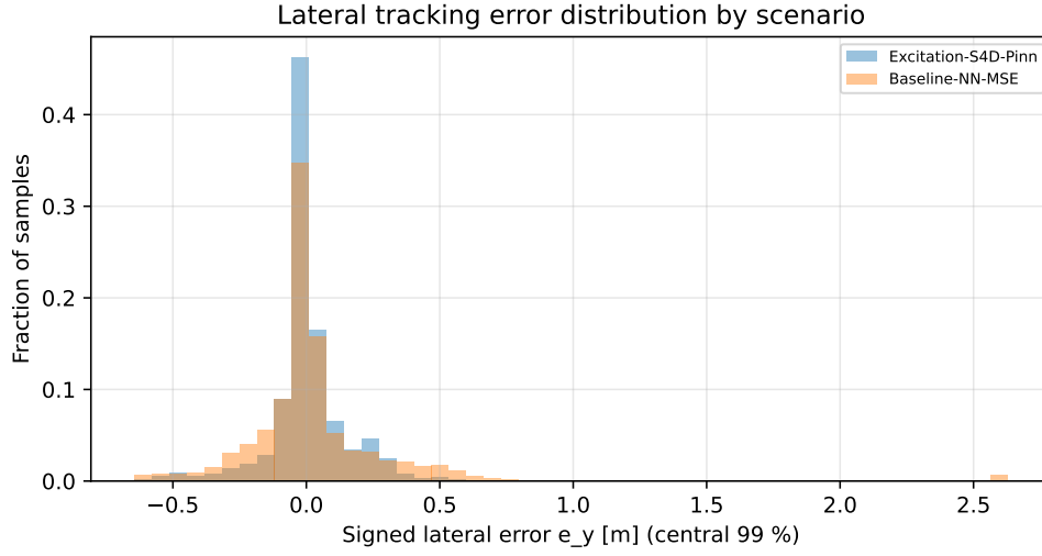
Fig. S10 Signed lateral tracking error over the whole run. The corrected configuration's distribution is narrower about a comparable centre, at sample standard deviation 0.256 m against 0.318 m and mean 0.021 m against 0.024 m, so the improvement is in spread, not in bias.
