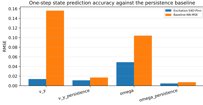
Fig. 6. One-step prediction RMSE for v_y and \omega against the persistence baseline of the same run. Neither identified model beats persistence at the 0.035 s model step.
