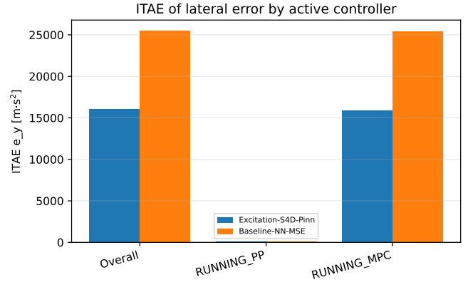
Fig. 11. ITAE of the lateral error, overall and split by the active controller. The pure-pursuit phases agree to 3 % and are two orders of magnitude smaller, so the whole difference sits in the MPC phase, where the identified model is in the loop.
