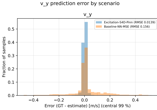
Fig. 7. Lateral-velocity prediction error (truth minus estimate). The corrected configuration is an order of magnitude tighter on this channel (0.014 m/s against 0.156 m/s RMSE), and neither model beats its own persistence baseline.
