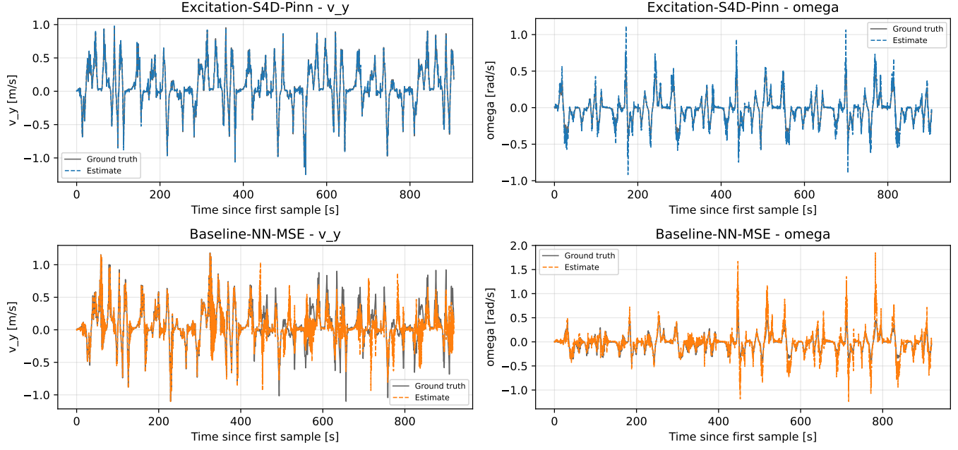
Estimated states against truth per scenario
