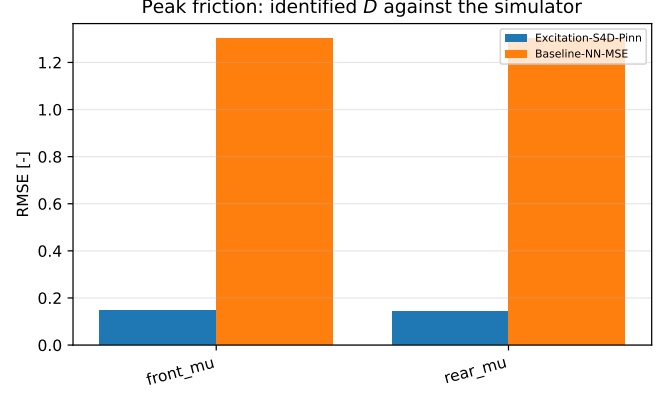
Fig. 2. Peak-friction error per axle against the effective coefficient the simulator reports per wheel, on the static \mu = 0.70 surface. The corrected configuration’s error is an order of magnitude smaller on both axes (0.145 and 0.142 against 1.300 on both, whole-run RMSE, and 0.078 once its friction gate has released); the inherited configuration’s error comes from a coefficient parked on its upper bound for the entire run rather than from a mis-estimate.
