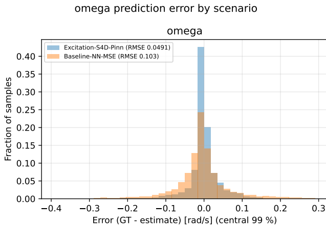
Fig. 8. Yaw-rate prediction error (truth minus estimate). The difference between the configurations is tail mass, not centre.
