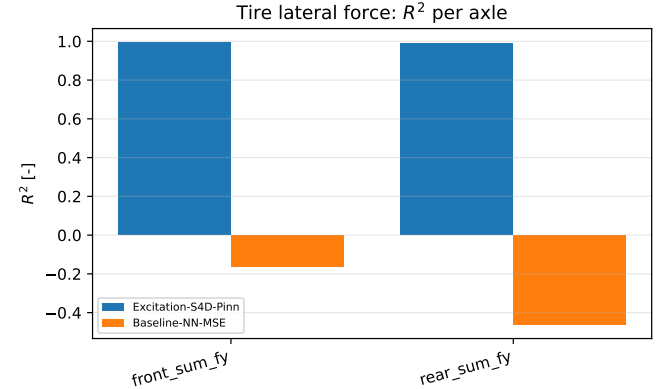
Fig. 3. Axle lateral force against the plant’s per-wheel telemetry, per axle: RMSE (top) and R^2 (bottom). The corrected configuration leads on both axes by an order of magnitude. The inherited configuration’s negative R^2 means its identified curve predicts the plant’s axle force worse than the mean of that force does, which is what a railed D = 2.0 does to the initial slope through (5) of the main paper.
