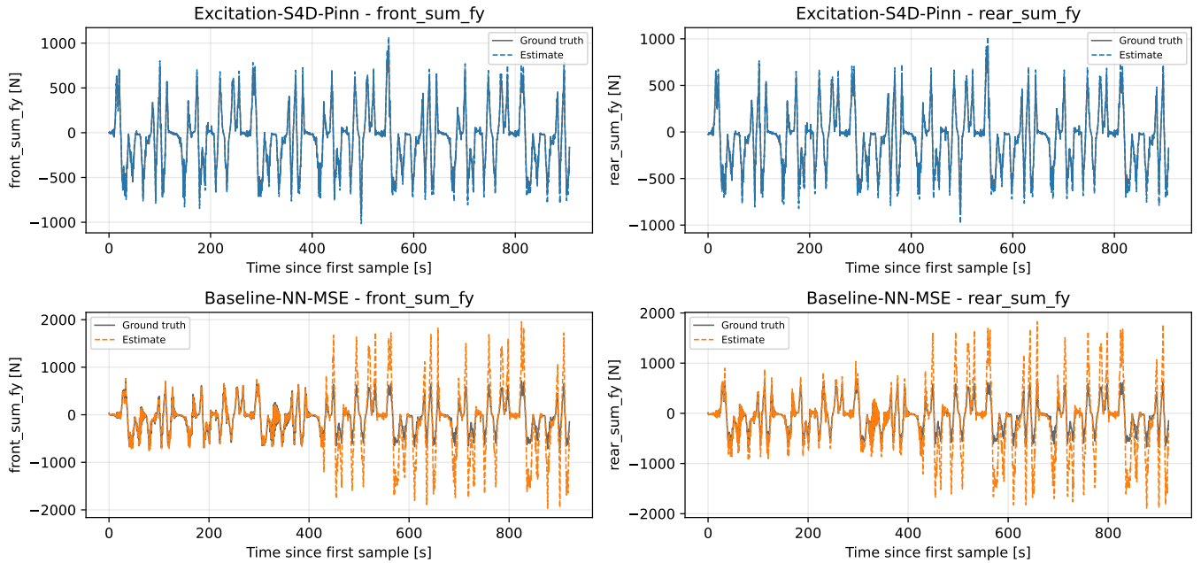
Tire lateral force: estimate against truth
