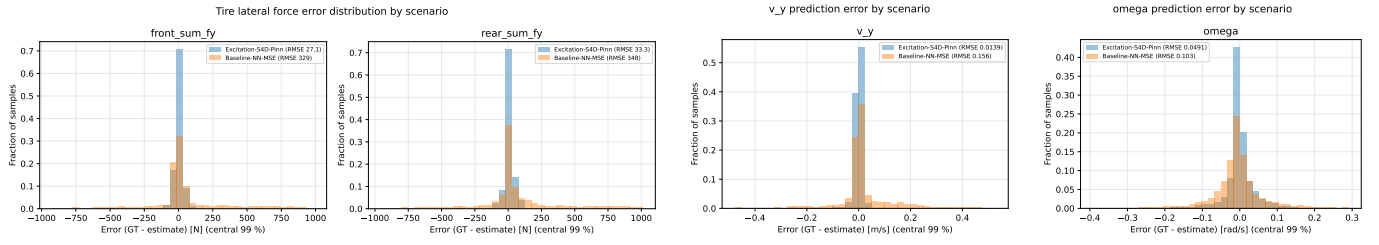
Fig. 6. Error distributions, truth minus estimate. (a) Axle lateral force, shared bin edges over the pooled central 99 % and normalised to each run’s sample count; both are centred, and Baseline-NN-MSE’s distribution is roughly an order of magnitude wider at every quantile (maximum absolute error 1249 N against 130 N front, 1219 N against 134 N rear). (b) One-step lateral velocity, where Excitation-S4D-Pinn is an order of magnitude tighter (0.014 m/s against 0.156 m/s RMSE). (c) One-step yaw rate, where the configurations differ in tail mass rather than centre. Neither model beats its own persistence baseline at the 0.035 s model step.
