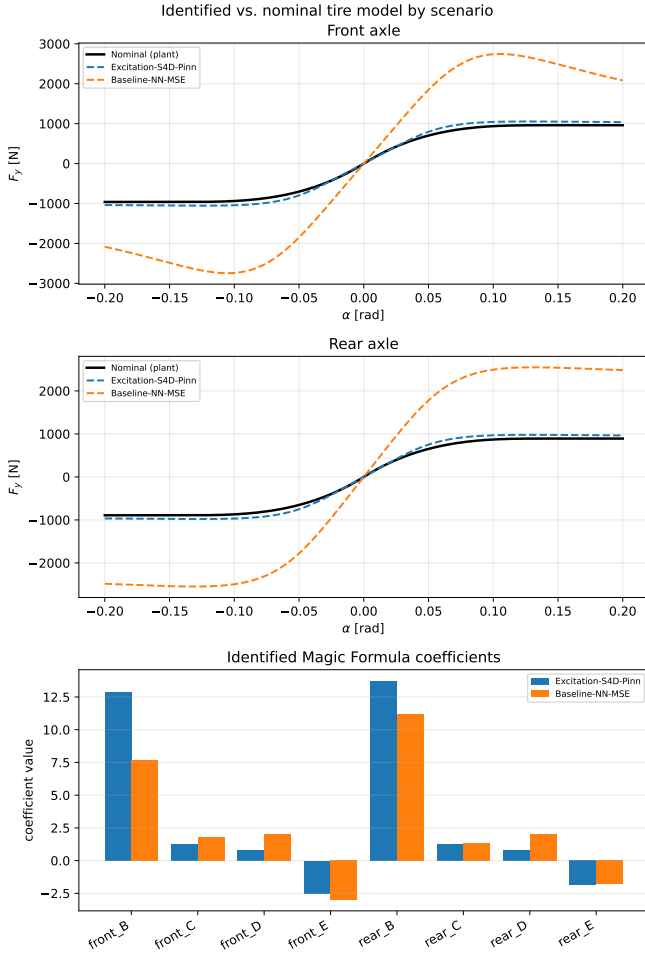
Fig. 4. Identified tire models against the plant. Top and middle: the plant's own curve (8) at the measured static load of each axle (black) against each run's last accepted identification. Bottom: the identified Magic Formula coefficients. Baseline-NN-MSE's accepted peak factor sits on its box constraint D = 2.0 on both axles in every cycle, so its curve carries roughly 2.8 times the plant's force at the edge of the plotted range, while Excitation-S4D-Pinn tracks both the plant's initial slope and its peak. All force metrics are axle sums.
