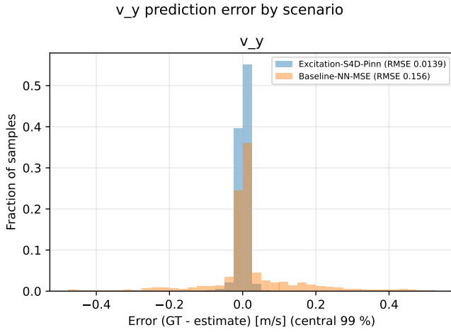
Fig. 7. Lateral-velocity prediction error (truth minus estimate). The corrected configuration is an order of magnitude tighter on this channel (0.014 m/s against 0.156 m/s RMSE), and neither model beats its own persistence baseline.
