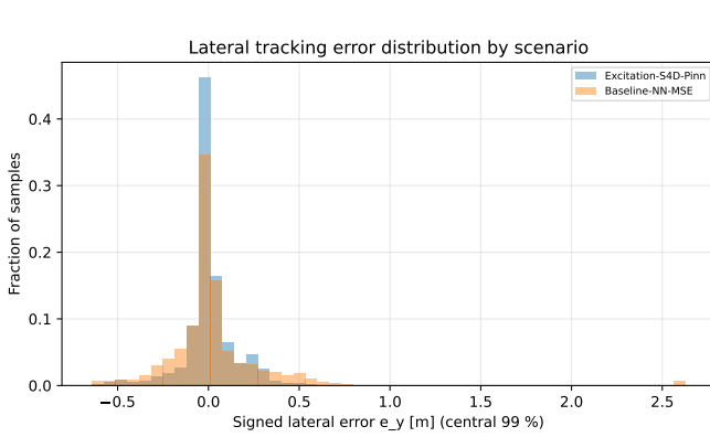
Fig. 10. Signed lateral tracking error over the whole run. The corrected configuration's distribution is narrower about a comparable centre, at sample standard deviation 0.256 m against 0.318 m and mean 0.021 m against 0.024 m, so the improvement is in spread, not in bias.
