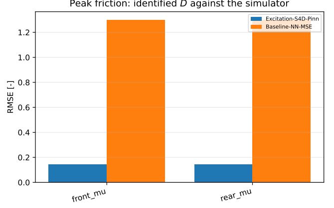
Fig. 2. Peak-friction error per axle against the effective coefficient the simulator reports per wheel ( \mu = 0.70 , static for both runs). The corrected configuration’s error is an order of magnitude smaller on both axles (0.145 and 0.142 against 1.300 on both, whole-run RMSE, and 0.078 once its friction gate has released); the inherited configuration’s error comes from a coefficient parked on its upper bound for the entire run rather than from a mis-estimate.
