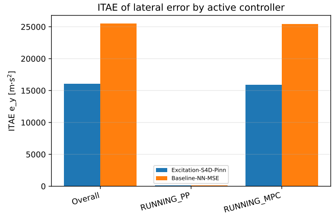
Fig. 11. ITAE of the lateral error, overall and split by the active controller. The pure-pursuit phases agree to 3 % and are two orders of magnitude smaller, so the whole difference sits in the MPC phase, where the identified model is in the loop.
