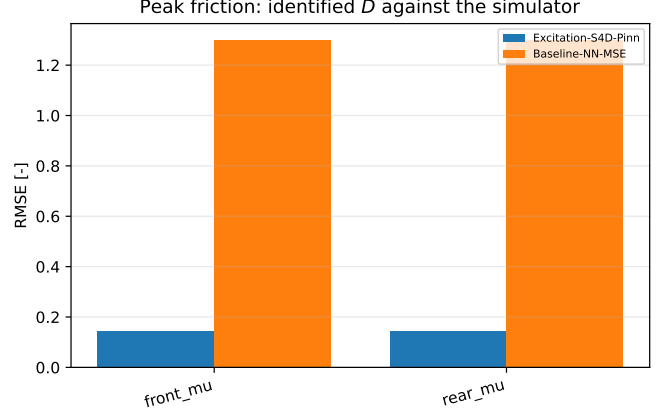
Fig. 2. Peak-friction error per axle against the effective coefficient the simulator reports per wheel ( \mu = 0.70 , static for both runs). The corrected configuration’s error is an order of magnitude smaller on both axles (0.145 and 0.142 against 1.300 on both, whole-run RMSE, and 0.078 once its friction gate has released); the inherited configuration’s error comes from a coefficient parked on its upper bound for the entire run rather than from a mis-estimate.
