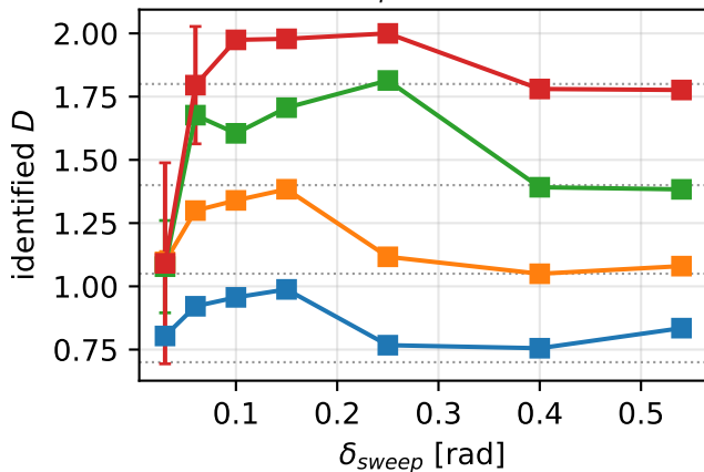
both axes against the bound
