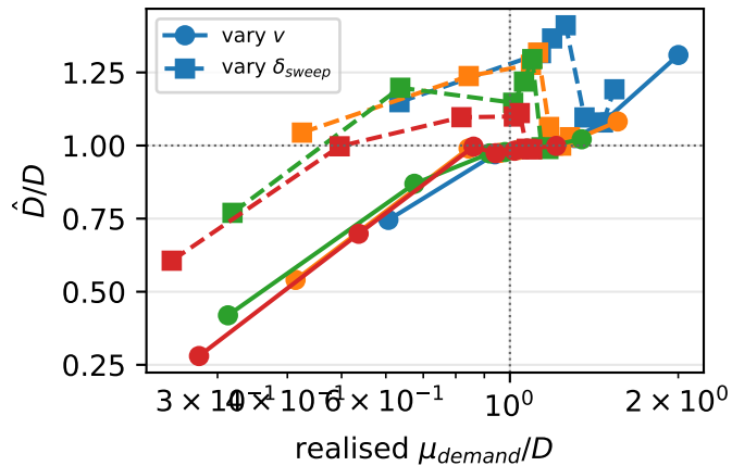
both axes against the bound
