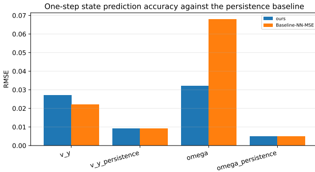
Fig. 13. One-step prediction RMSE for v_y and \omega against the persistence baseline of the same run. Neither identified model beats persistence at the 0.035 s model step.
