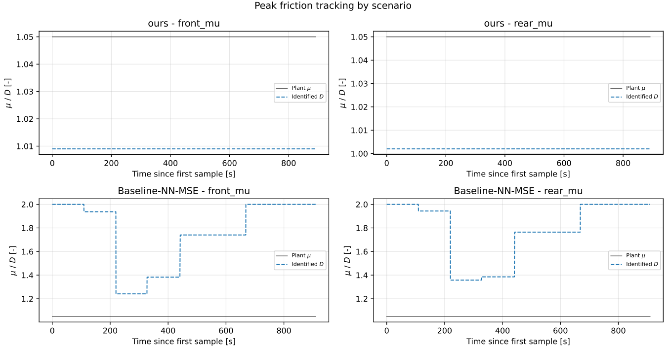
Fig. 9. Peak friction over the run, one row per configuration: the plant’s effective \mu (black) against the identified peak factor D published at each of the six accepted identifications. The surface is static, so every departure from the black line is estimator error. Ours is a flat line about 0.04 below the plant on both axes—the same coefficients every cycle—while Baseline-NN-MSE starts and ends on the D \leq 2.0 box constraint and does not settle in between.
