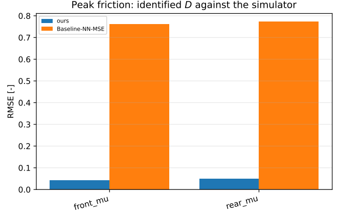
Fig. 8. Peak-friction error per axle against the effective coefficient the simulator reports per wheel ( \mu = 1.05 , static for both runs). The corrected configuration's error is an order of magnitude smaller on both axles (0.041 and 0.048 against 0.762 and 0.772 RMSE); the inherited configuration's error is not a mis-estimate but a coefficient parked on its upper bound.
