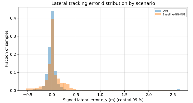
Fig. 18. Signed lateral tracking error over the whole run. The corrected configuration's distribution is narrower about a comparable centre—sample standard deviation 0.279 m against 0.301 m, mean 0.014 m against 0.039 m—so the improvement is in spread, not in bias.
