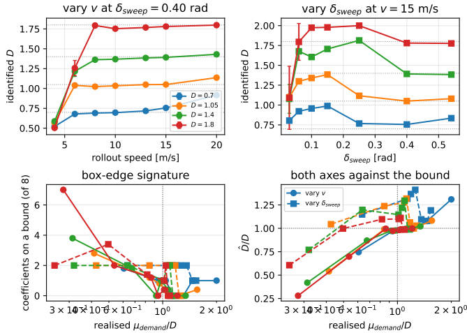
Fig. 6. The grid of Table V. Top: recovered peak factor against rollout speed (left, \delta_{\text{sweep}} = 0.4 rad) and against sweep amplitude (right, v = 15 m/s), one series per true D (dotted lines), mean \pm 95% interval over the noise realisations. Bottom: the same fits against the demand the rollout actually realises, \max |v_x \omega|/g , normalised by the tire's own D ; left, the mean number of coefficients on a box constraint, right, \hat{D}/D . Below a realised demand of D (dotted vertical) the fit reports the excitation and not the tire on both axes—downward when the speed is the limiting factor, upward when the sweep amplitude is—and the coefficients slide onto the box.
