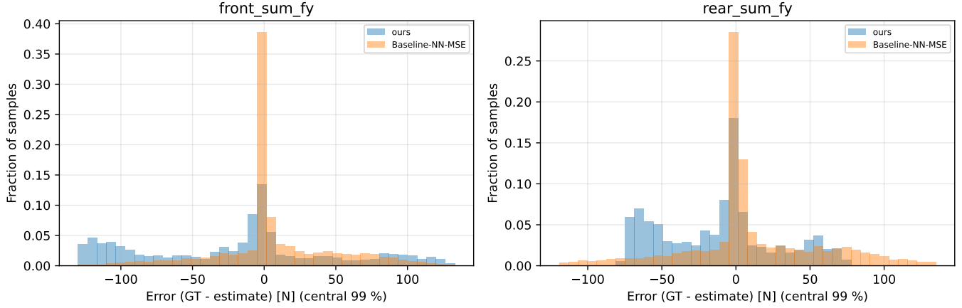
Fig. 11. Distribution of the axle lateral-force error (truth minus estimate), shared bin edges over the pooled central 99% and normalised to the sample count of each run. Both are centred; the inherited configuration buys its lower front RMSE with the heavier tail (maximum absolute error 215 N against 138 N front, 223 N against 85 N rear).
