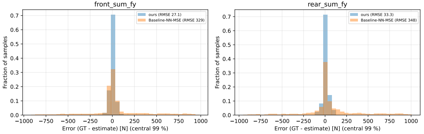
Fig. 4. Distribution of the axle lateral-force error (truth minus estimate), shared bin edges over the pooled central 99% and normalised to the sample count of each run. Both are centred, and the inherited configuration's distribution is roughly an order of magnitude wider at every quantile (maximum absolute error 1295 N against 264 N front, 1316 N against 135 N rear).
