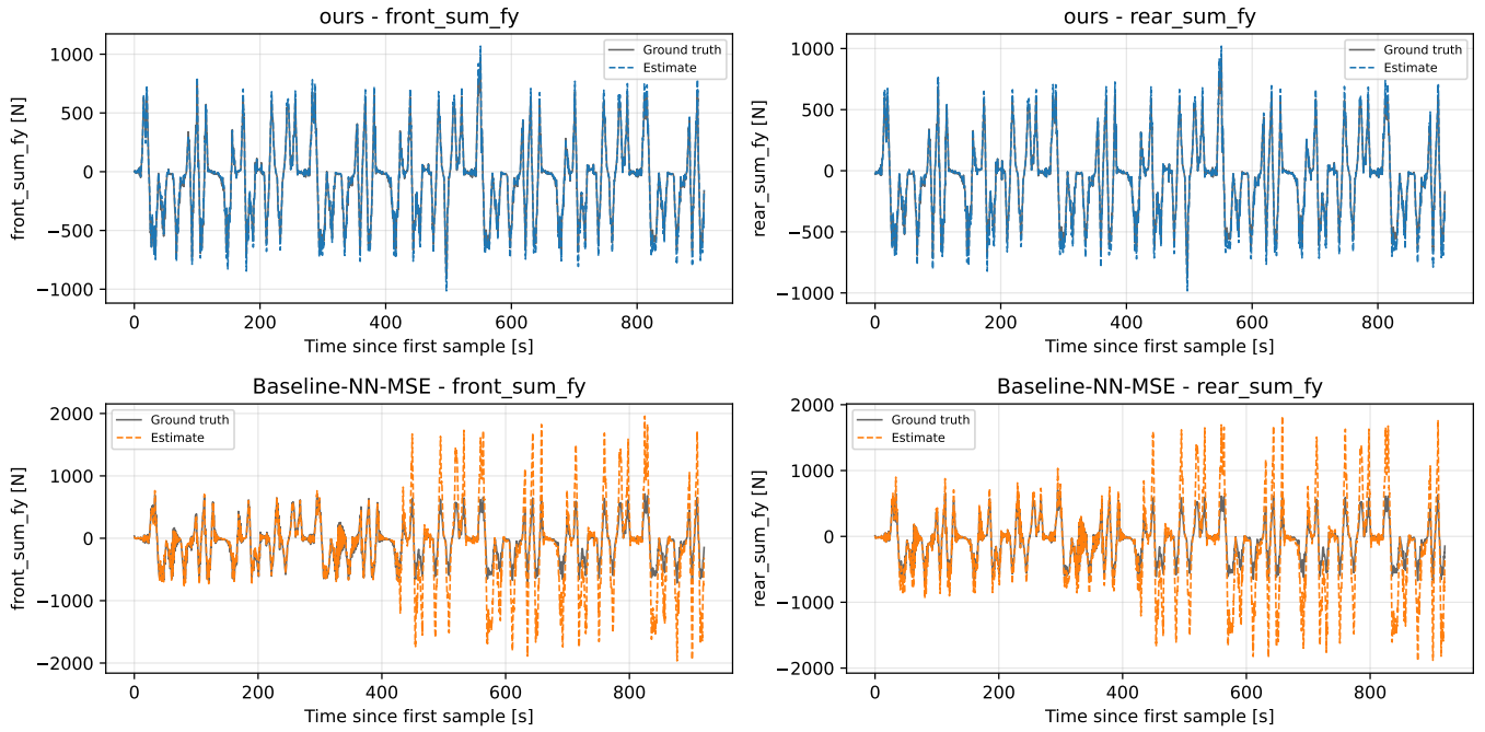
Tire lateral force: estimate against truth
