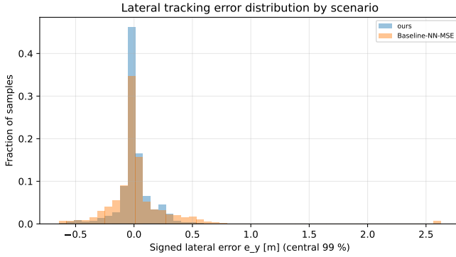
Fig. 10. Signed lateral tracking error over the whole run. The corrected configuration's distribution is narrower about a comparable centre, at sample standard deviation 0.256 m against 0.318 m and mean 0.021 m against 0.024 m, so the improvement is in spread, not in bias.
